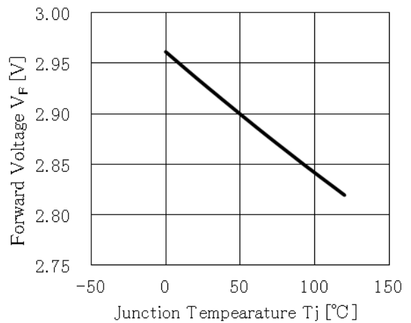
Forward Voltage vs Junction Temperature ( I_F=65\text{mA} )
