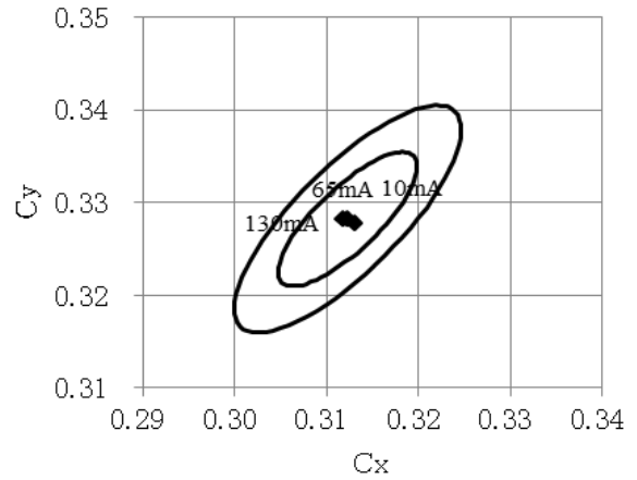
Chromaticity vs Forward Current (Ta=25°C)
