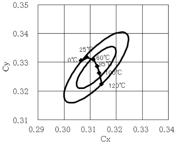
Chromaticity vs Junction Temperature ( I_F=65\text{mA} )
