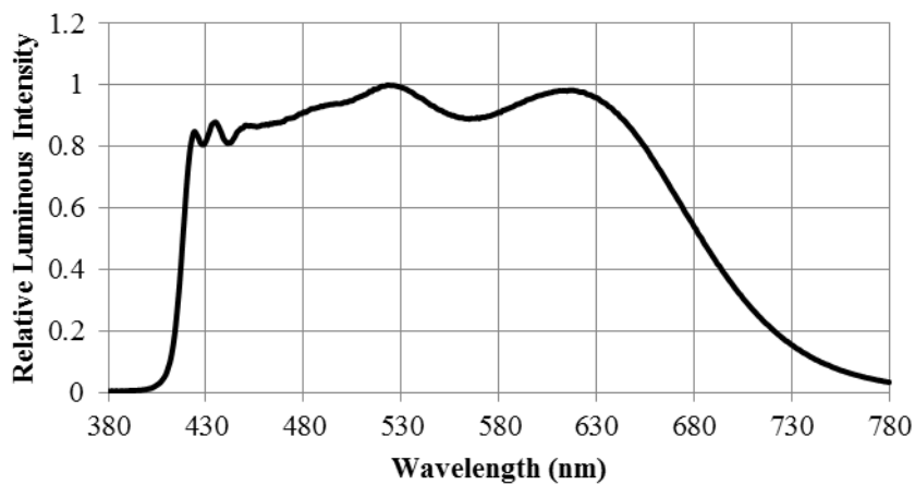
Spectrum (Ta=25°C, If=65mA)
